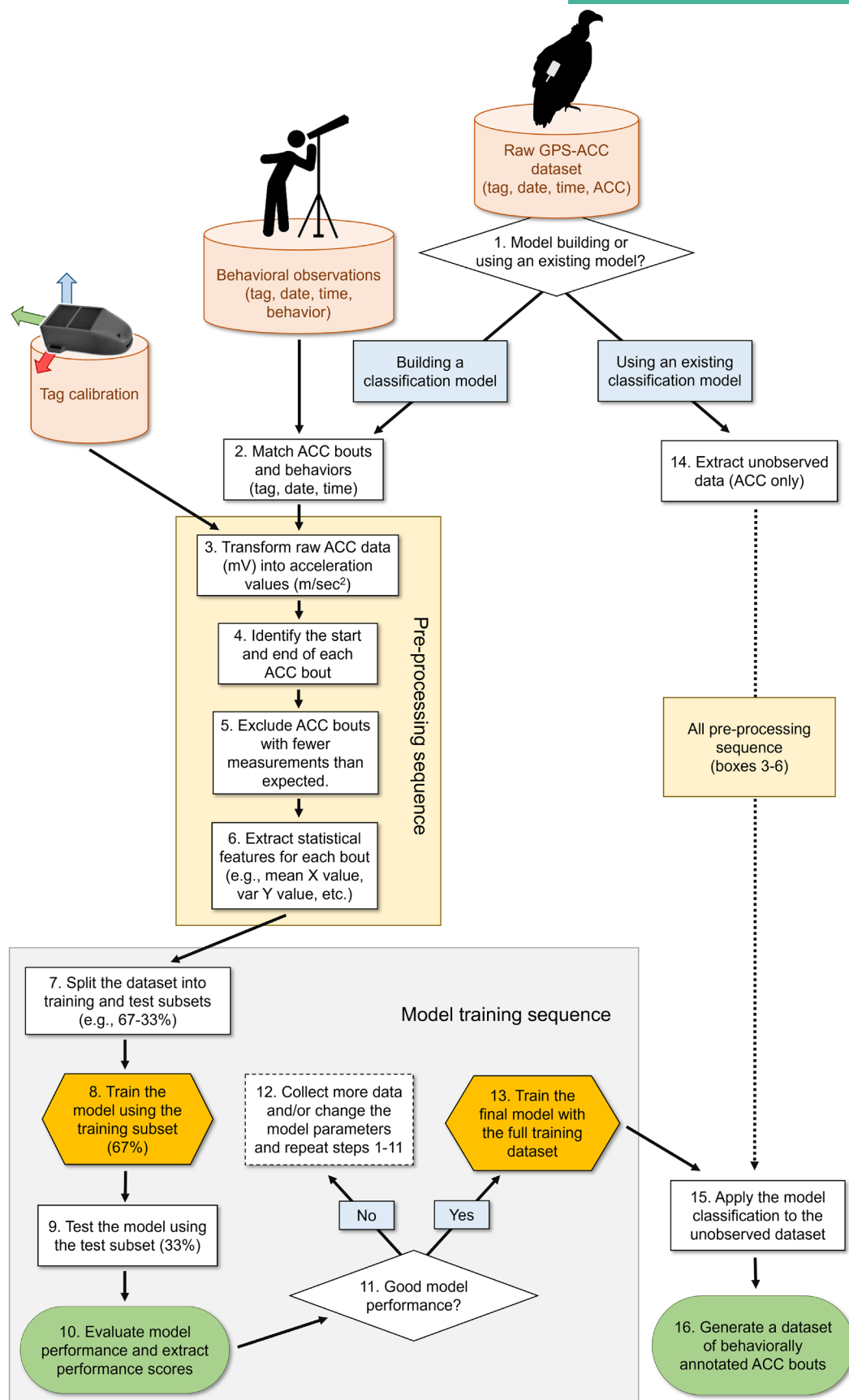
FIGURE 2 Methodological workflow outlining the process of identifying behaviours of wild animals based on accelerometer data. All the training data, code and tutorials necessary to follow this workflow are available on GitHub ( www.github.com/Orrslab/ACC_behavior_classification ) and at (Acácio et al., 2025).
