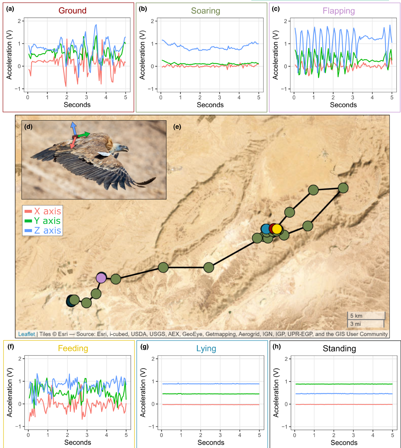
FIGURE 1 Examples of accelerometer-based classification of griffon vulture's behaviours. Acceleration measurements of bouts classified as: (a) 'Ground', (b) 'Soaring' flight, (c) 'Flapping' flight, (f) 'Feeding', (g) 'Lying' and (h) 'Standing'. The acceleration data was collected at 20Hz during 5 s for three orthogonal axes (d): Sway—X (red), surge—Y (green), and heave—Z (blue). (e) GPS tracking of a griffon vulture over 1 day. The colours of the GPS locations match the behaviours recorded on that location: 'Ground'—red; 'Soaring'—green; 'Flapping'—violet; 'Feeding'—yellow; 'Lying'—light blue; 'Standing'—black. This illustrates the large daily movements of griffon vultures, emphasizing the logistical challenges associated with surveillance in the desert study area. Photo credit: Yacov Ben Bunan.
