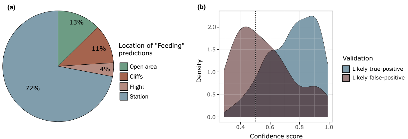
FIGURE 5 Validation of 'Feeding' behaviours using data from free-roaming griffons. (a) Percentage of 'Feeding' predictions ( n = 175 ) located within a supplementary feeding station ('Station'—blue), on open landscape ('Open area'—green), on cliffs ('Cliffs'—dark brown) or in flight ('Flight'—light brown). (b) Distribution of the confidence scores of 'Feeding' bouts likely to be true-positives (located within a feeding station, in blue) and likely to be false-positives (located on cliffs or in flight, in dark red). The dashed line indicates the confidence threshold of 0.5, a conservative threshold that reduces the number of false-positives, while including nearly all true-positive predictions.
